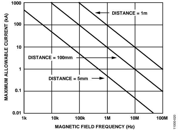
Figure 20. Maximum Allowable Current for Various Current-to-ADuM340xW Spacings
