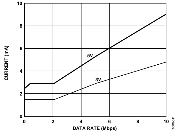
Figure 11. Typical ADuM3400W V_{DD1} Supply Current vs. Data Rate for 5 V and 3 V Operation
