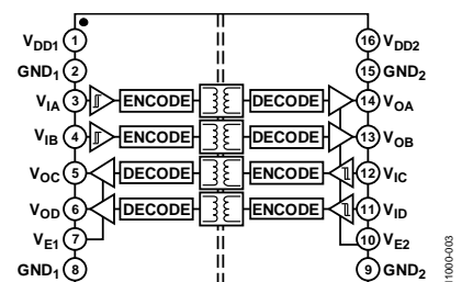
Figure 3. ADuM3402W Functional Block Diagram
