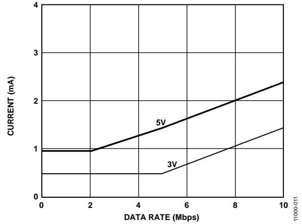
Figure 12. Typical ADuM3400W V_{DD2} Supply Current vs. Data Rate for 5 V and 3 V Operation
